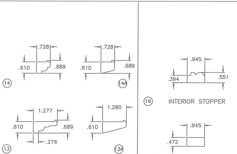
GLAZING BEADS ⑬ ⑭ ⑮ ⑯ ⑰ MIDDLE STOPPER
