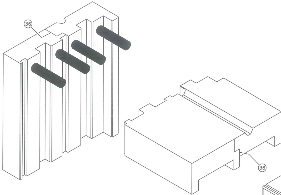
RECT. FRAME TOP CORNER
