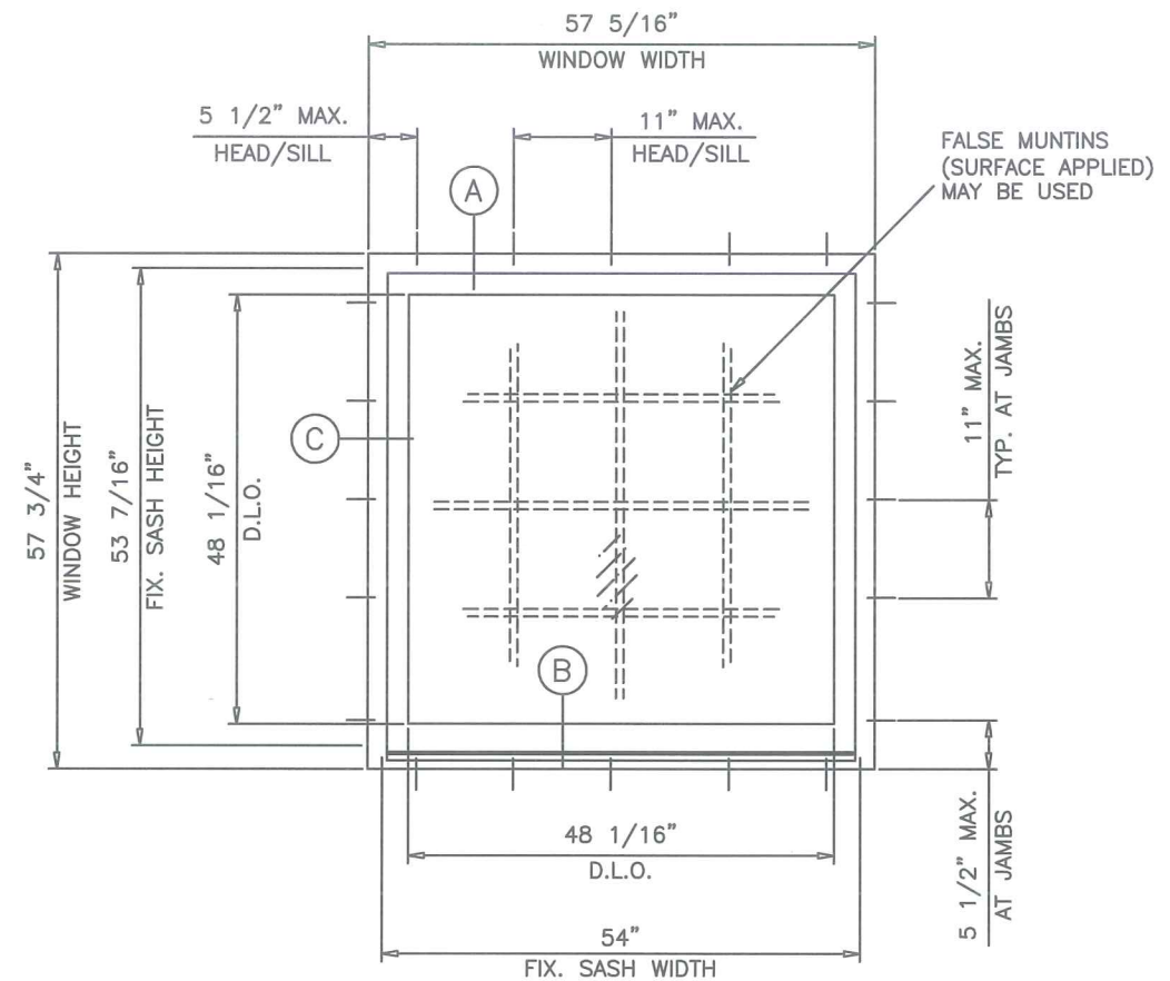
TYPICAL ELEVATION
