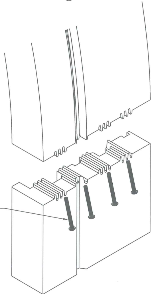
CIRCULAR FRAME CORNER
