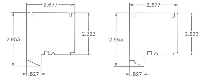
⑦ FIXED UPPER SASH OPTIONAL
